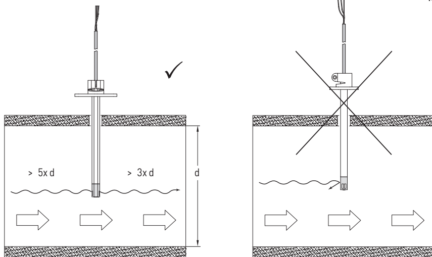
Mounting diagram
